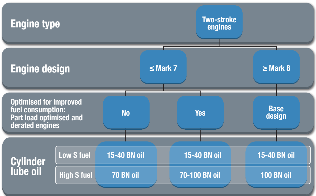
Fig. 1: General overview of cylinder lube oils and how to choose a suitable cylinder lube oil. Low S fuel = low-sulphur fuel incl. distillates, new types of fuels with less 0.1% S (ULSFO), LNG, methanol, ethane and LPG. High S fuel = high-sulphur fuel
